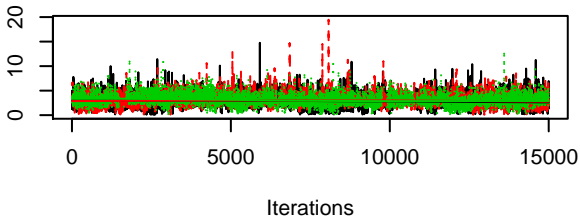
Trace of gamma0[2]
