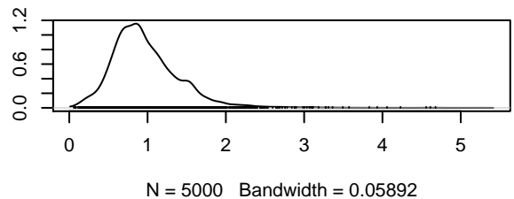
Density of beta0[4]
