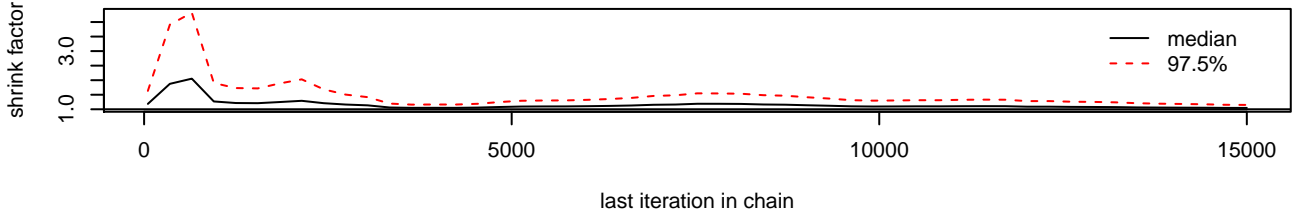
tau0[1]
