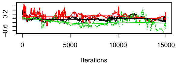
Trace of mu0[3]
