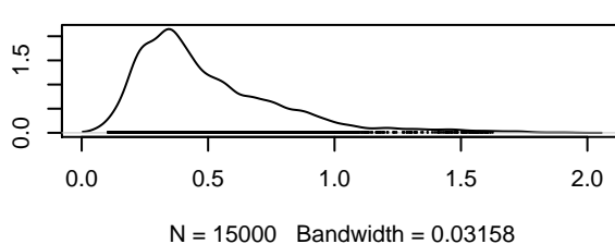
Density of beta0[3]
