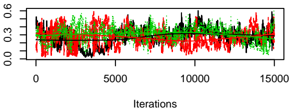
Trace of alpha0[2]
