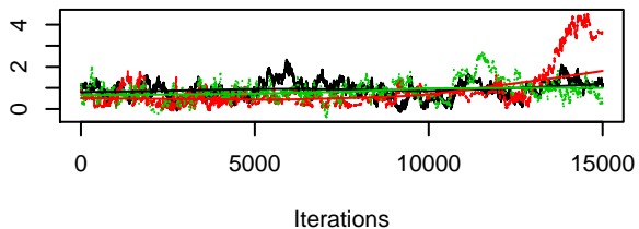
Trace of mu0[4]
