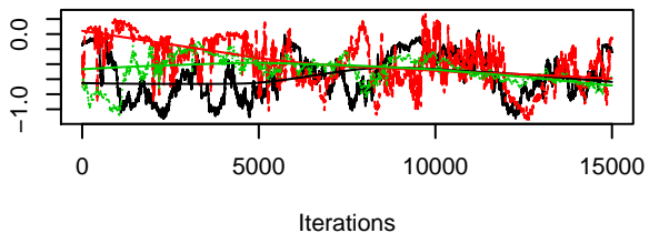
Trace of mu0[2]
