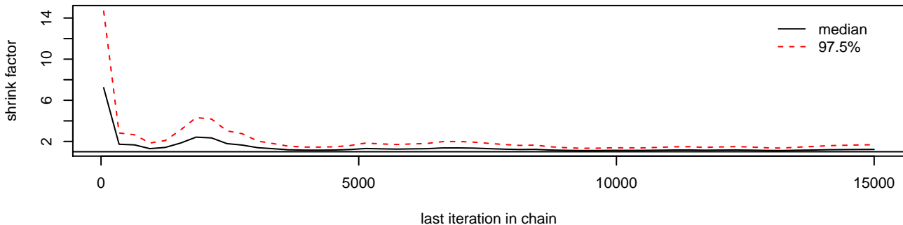
tau0[1]
