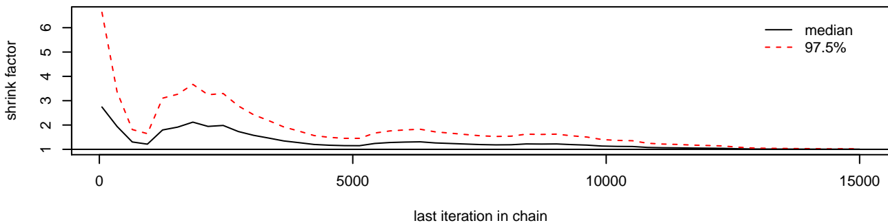
tau0[3]
