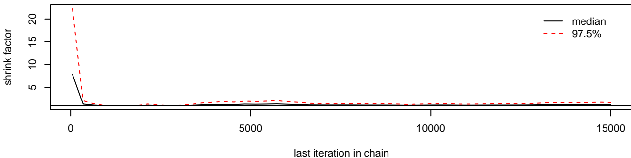
tau0[2]
