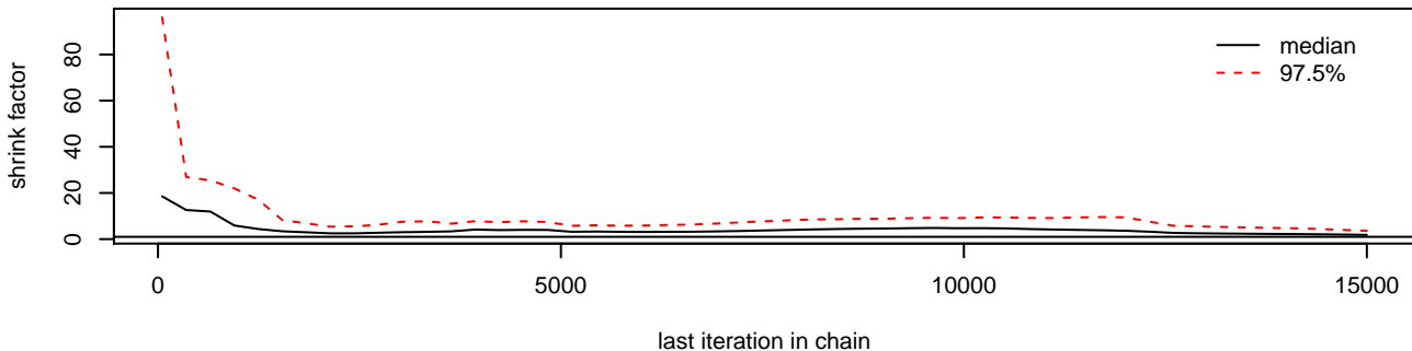
beta0[1]
