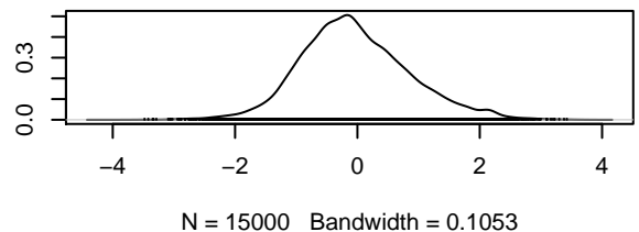
Density of tau0[4]
