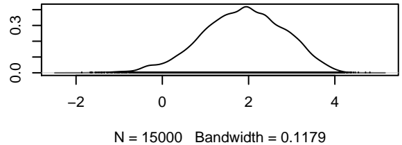
Density of tau0[2]
