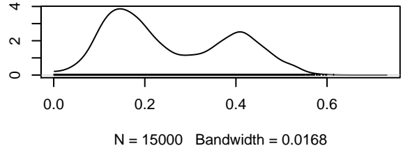
Density of alpha0[3]
