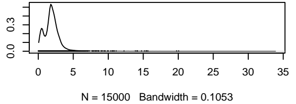
Density of gamma0[1]
