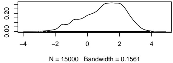
Density of tau0[1]
