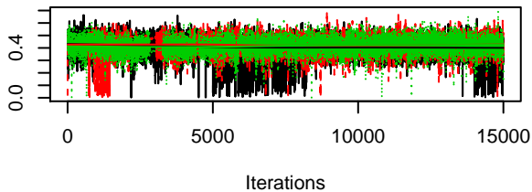
Trace of alpha0[2]
