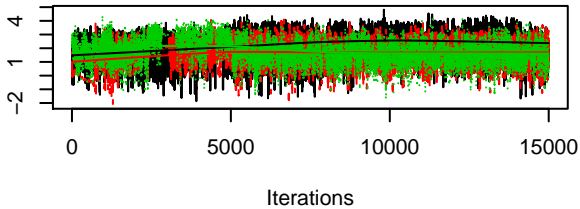
Trace of tau0[2]
