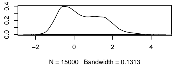
Density of tau0[3]
