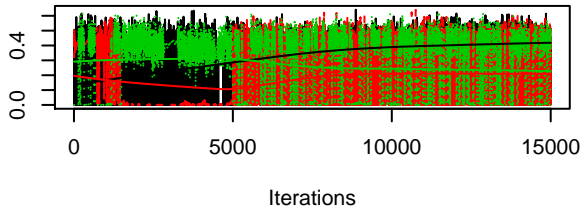
Trace of alpha0[1]
