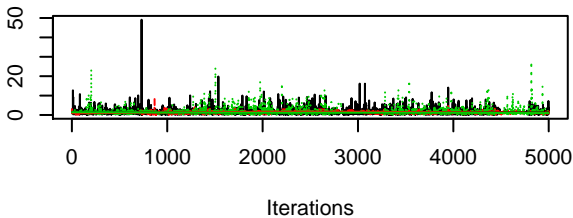
Trace of gamma0[4]
