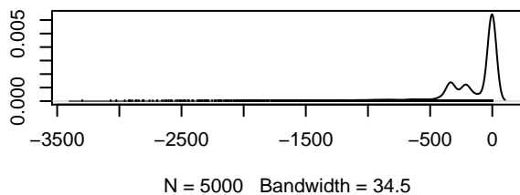
Density of mu0[1]
