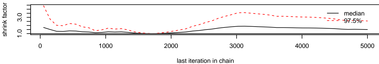
tau0[1]
