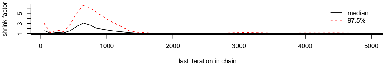
beta0[3]
