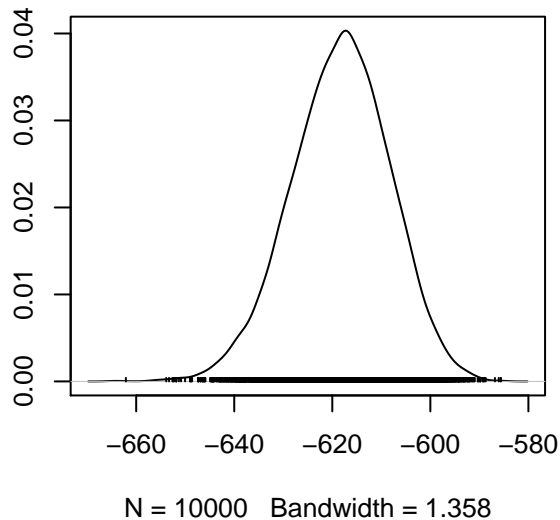
Density of l_p __
