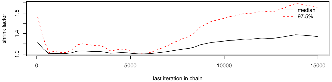
tau0[1]
