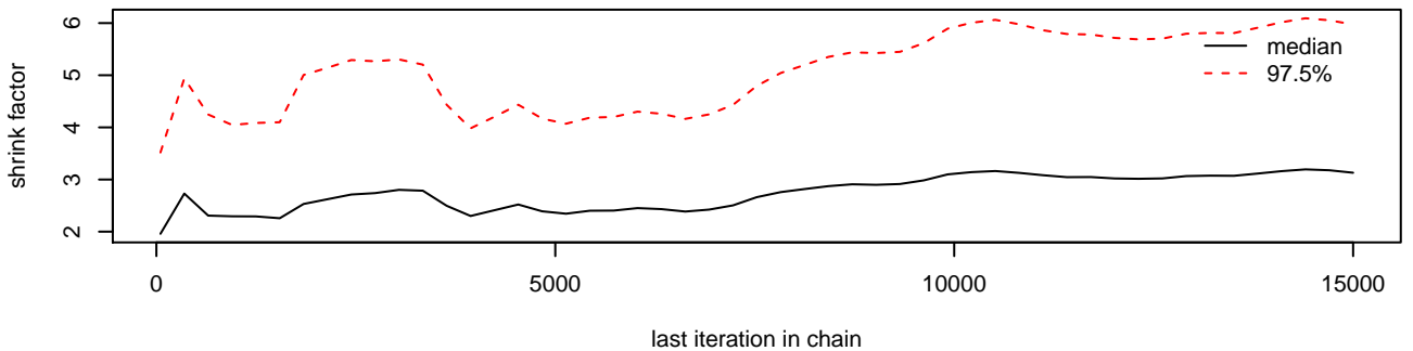
tau0[3]
