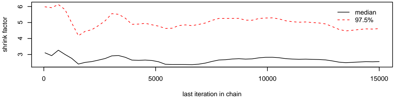
tau0[2]
