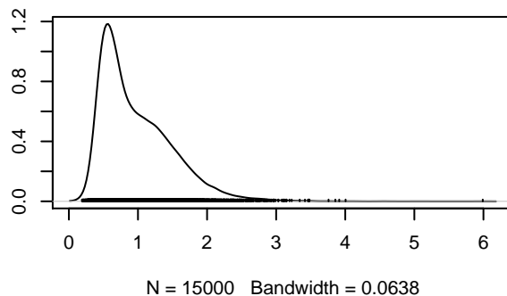
Density of beta0[2]
