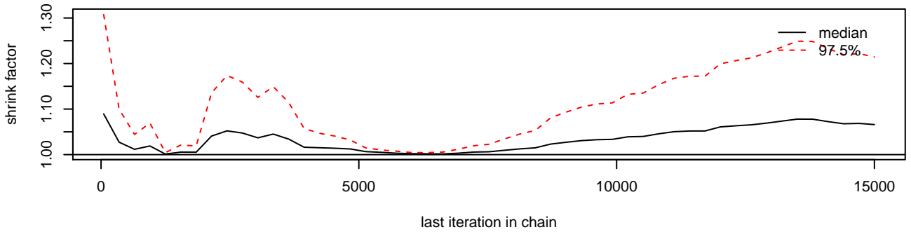
gamma0[1]
