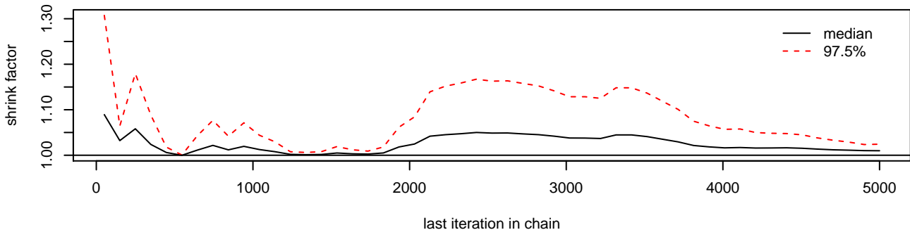
gamma0[1]
