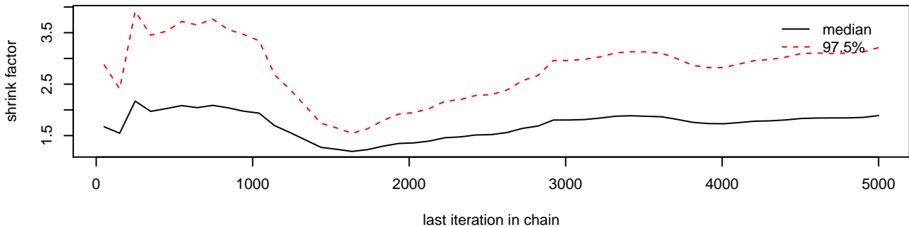
gamma0[2]
