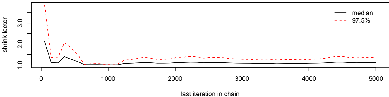
gamma0[3]
