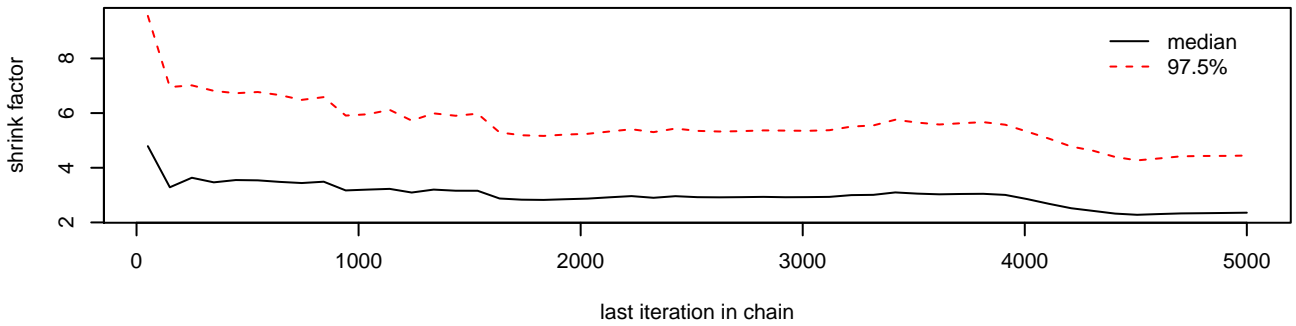
alpha0[3]
