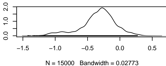
Density of mu0[2]
