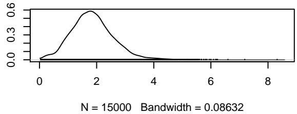
Density of gamma0[2]
