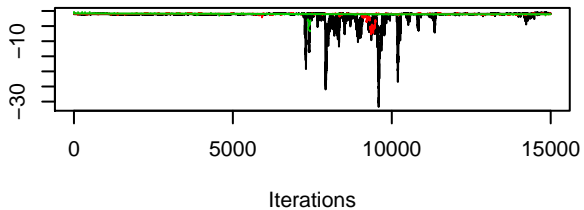
Trace of mu0[1]
