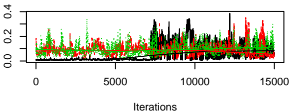
Trace of alpha0[4]
