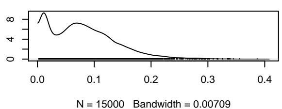
Density of alpha0[4]
