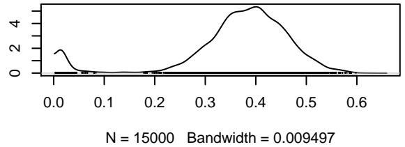
Density of alpha0[1]
