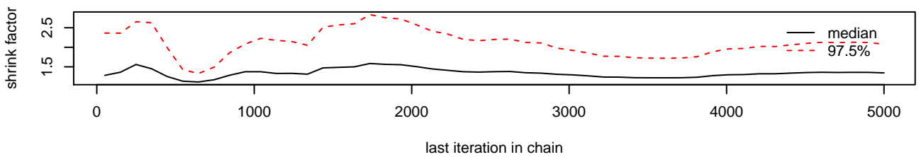
tau0[3]
