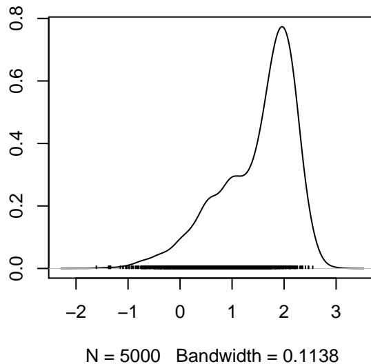
Density of tau0[1]
