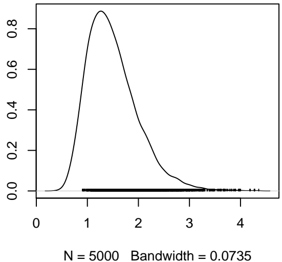
Density of gamma0[2]
