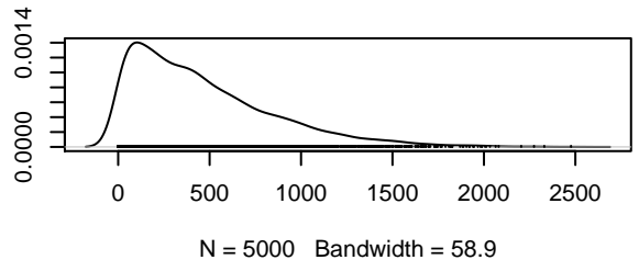
Density of mu0[3]
