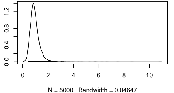
Density of beta0[2]
