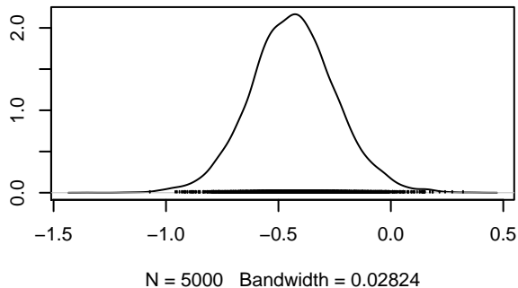
Density of \mu_0[1]
