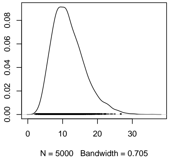
Density of alphaN
