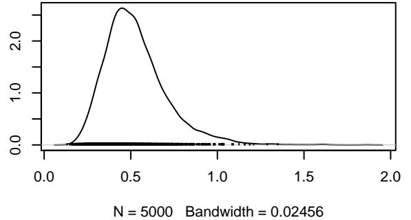
Density of beta0[1]
