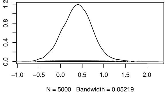
Density of \mu_0[2]
