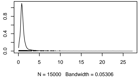
Density of gamma0[1]
