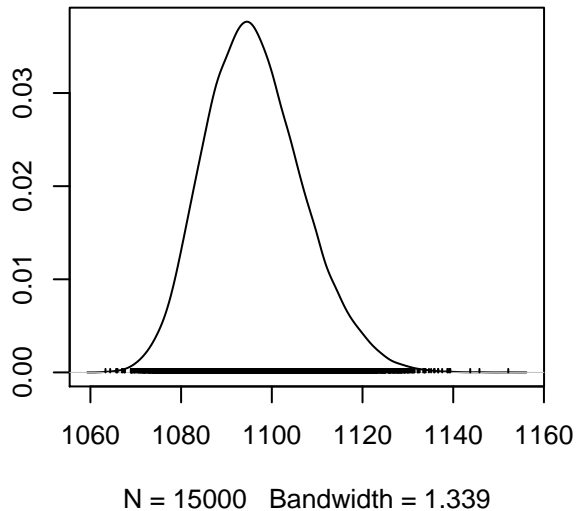
Density of deviance
