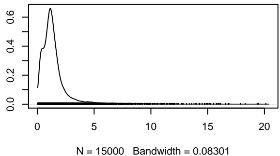
Density of gamma0[3]
