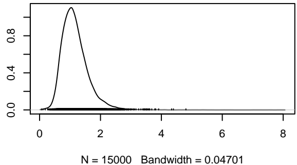
Density of gamma0[2]
