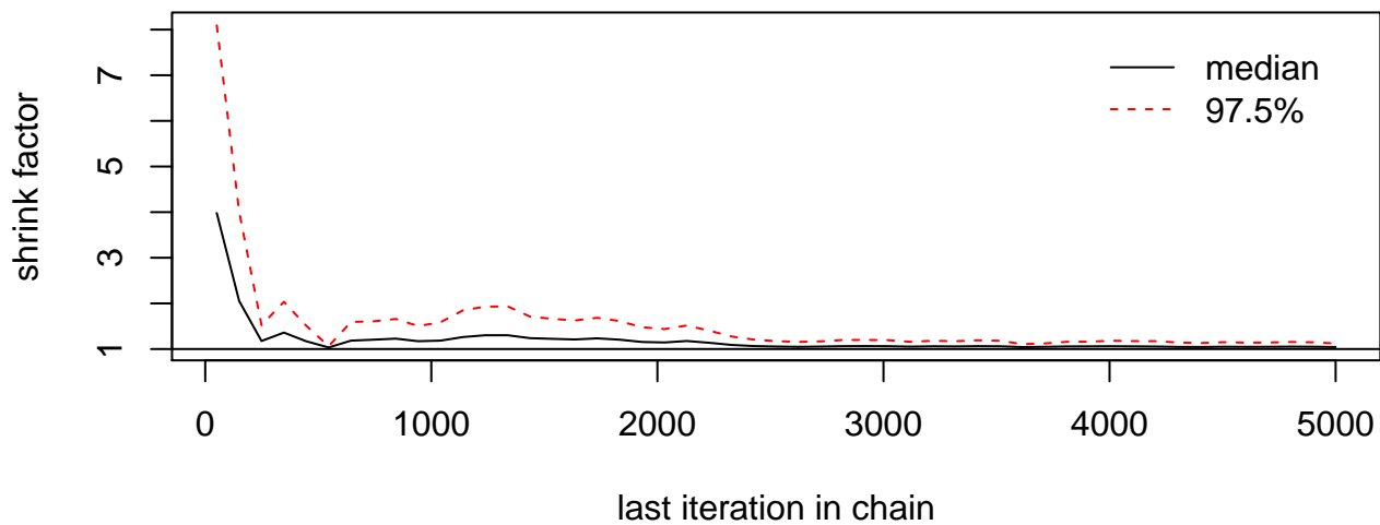
gamma0[2]
