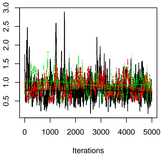
Trace of beta0[2]
