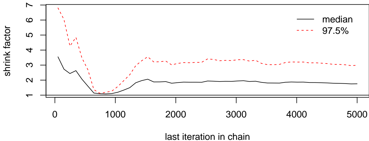
gamma0[1]
